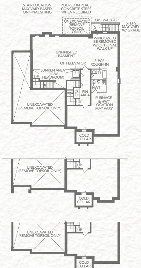
ELEVATION A, B, C BASEMENT
