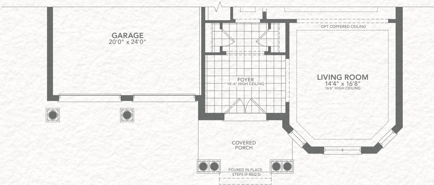
ELEVATION C | MAIN FLOOR
