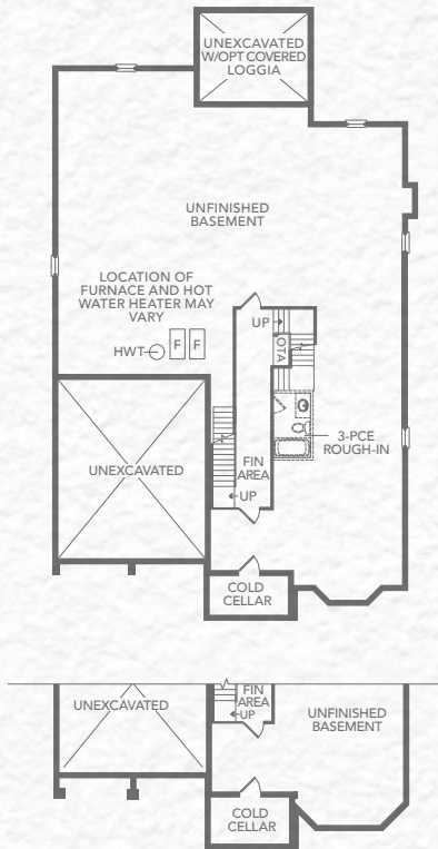
ELEVATION B, C BASEMENT
