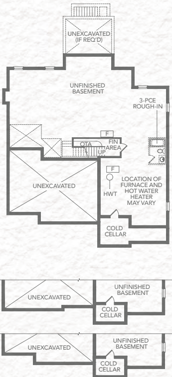
ELEVATION A, B, C BASEMENT
