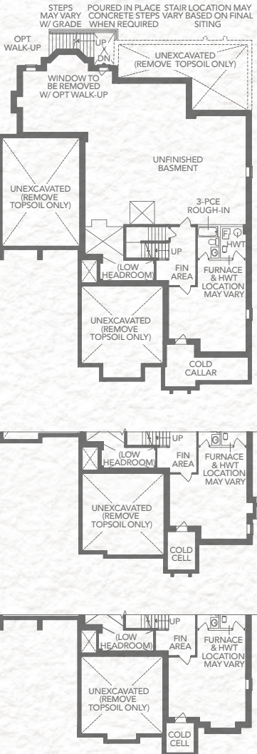
ELEVATION A, B, C BASEMENT
